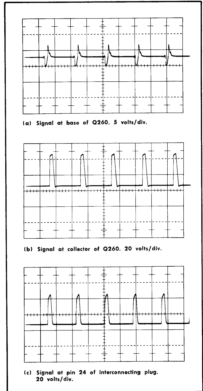
Fig. 3-2. Signals in blocking oscillator circuit. Test oscilloscope ac coupled at sweep rate of 2 \mu\text{sec}/\text{division} .
