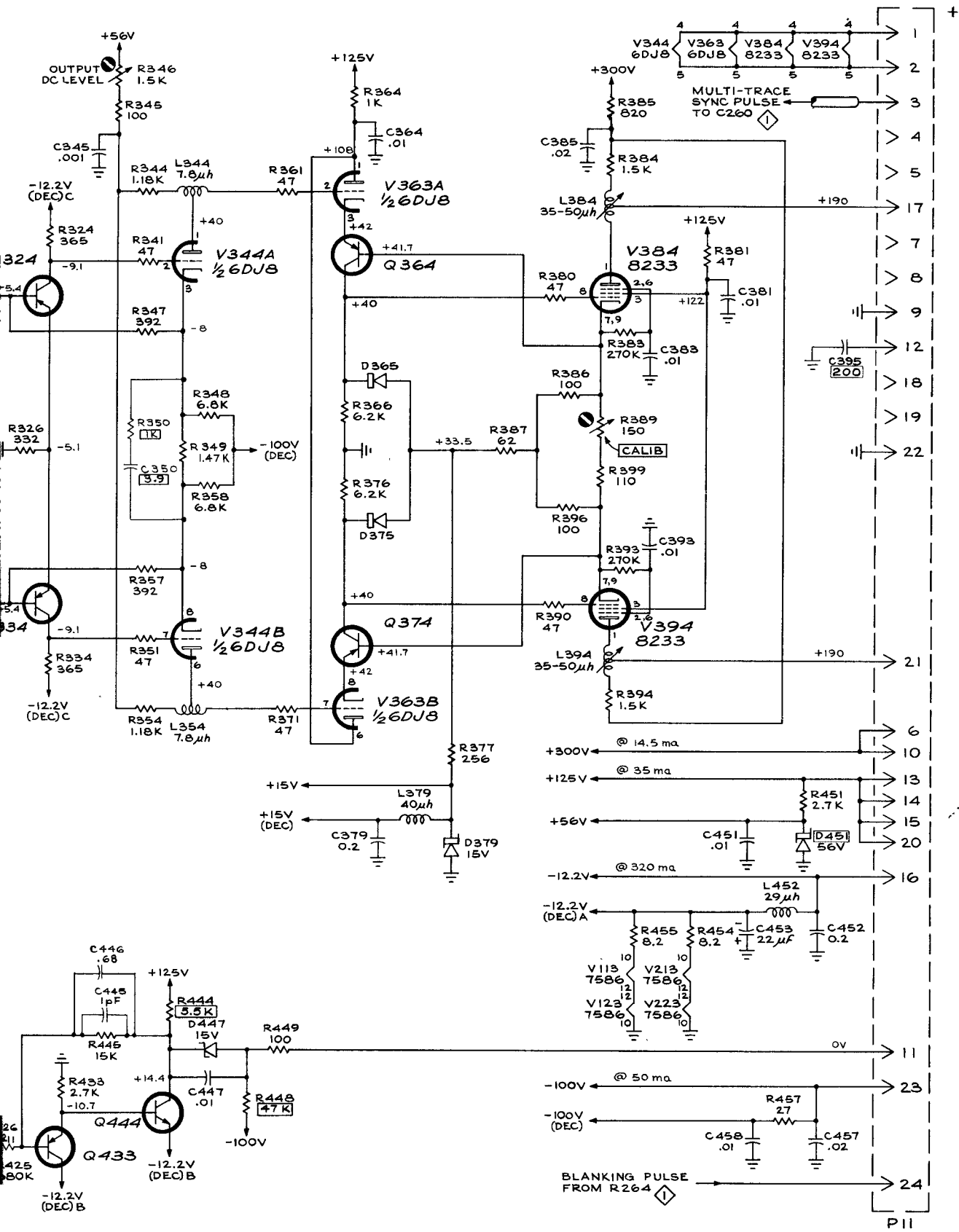
269 OUTPUT AMPLIFIER
